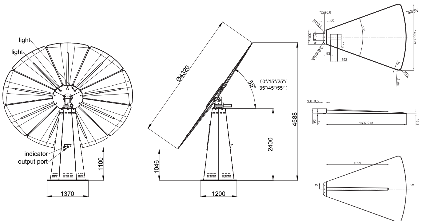
Figure 1. Dimension and diameter HEX3000
