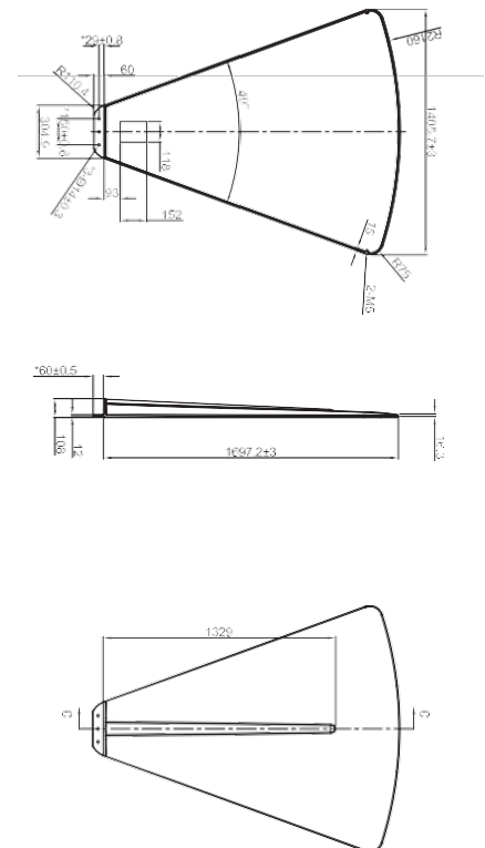
Figure 2. Dimension solar panel
